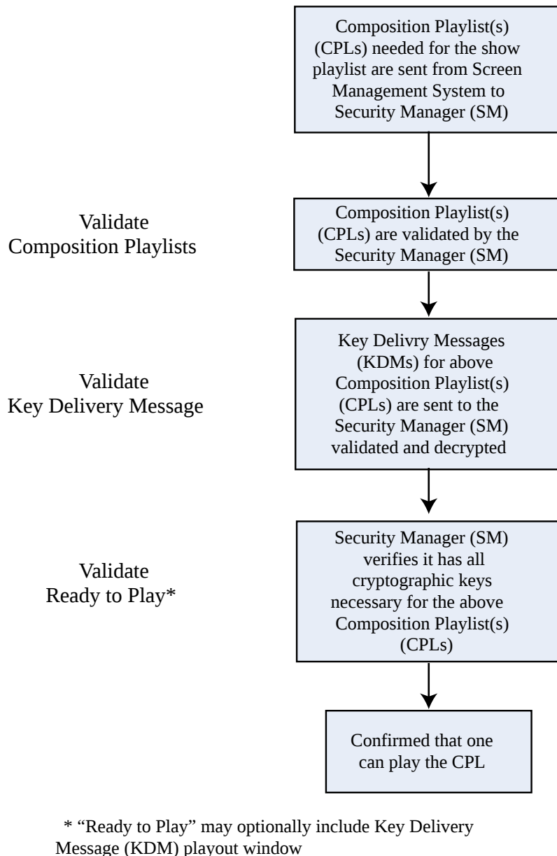
Figure 17: Pre-Show Overview
